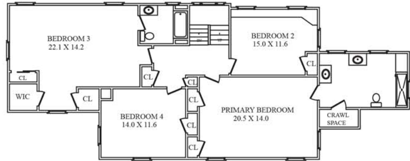
SECOND FLOOR
