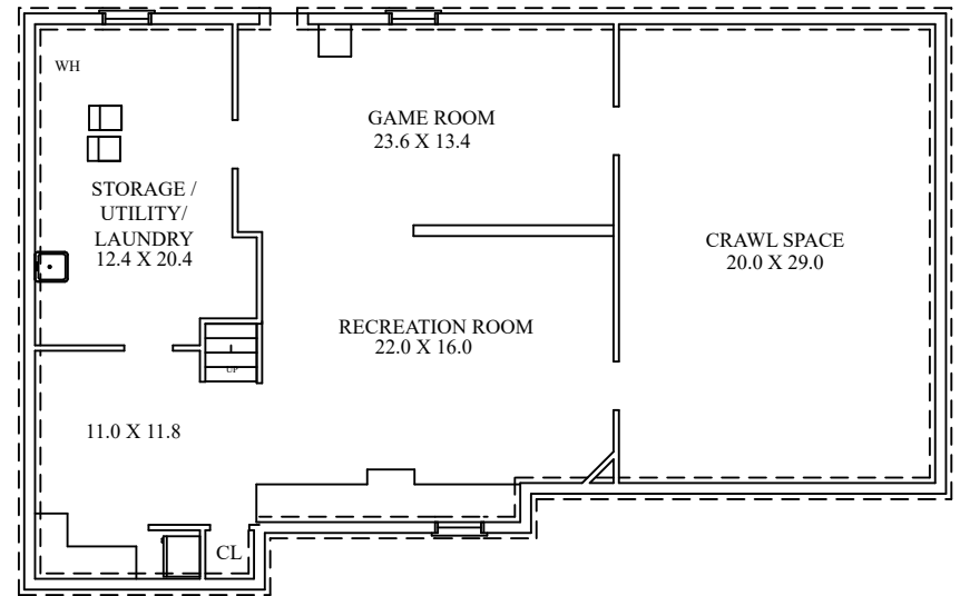
LOWER LEVEL
